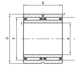
NAO...W double row
