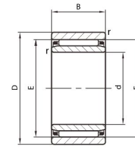
NAO single row
