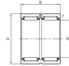
RNA 69 ( dr \geq 40mm ) double row
