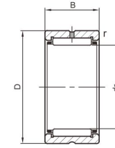
NK (dr≥12) NKS ,RNA 49 ,RNA 59 RNA 69 (dr≤35) single row
