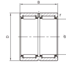
RNA 69 (dr≥40mm) double row
