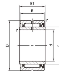
NA49...2RS
