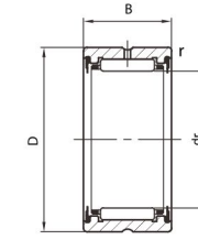
NA69...2RS
