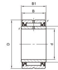
RNA69...2RS
