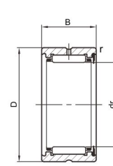
RNA49...2RS
