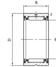
NA69...2RS
