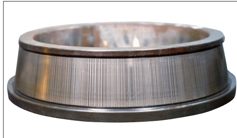
Photo 15-1 Part: Inner ring of a tapered roller bearing Symptom: Striped pattern of erosion on the raceway surface
