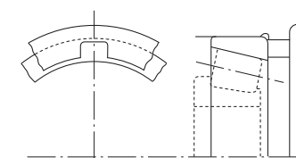
Fig. 1.11 Removal Notches
