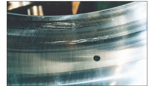
Photo 4-6 Part: Outer ring of Photo 4-5 Symptom: Partial smearing circumferentially on raceway surface Cause: Poor lubrication
