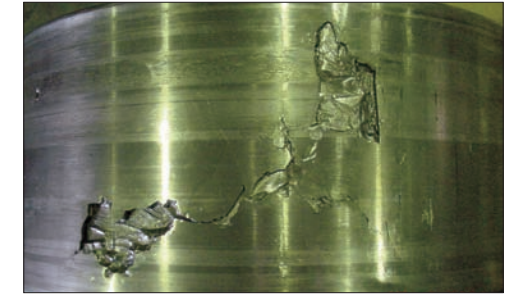
Photo 1-12 Part: Outer ring of a cylindrical roller bearing for Sendzimir mills Symptom: Flaking of outside surface Cause: Progression of fatigue in outer ring material (Prolonged grinding on outer ring outside surface)
