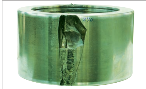
Photo 6-4 Part: Outer ring of a double-row cylindrical roller bearing (outer ring rotation) Symptom: Cracks on outside surface Cause: Flat wear and heat generation due to non-rotation of the outer ring
