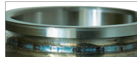
Photo 13-3 Part: Inner ring of an angular contact ball bearing Symptom: Raceway discoloration, melting at ball pitch intervals Cause: Excessive preload
