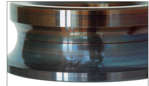
Photo 18-2 Part: Inner ring of a four-point contact ball bearing Symptom: Bluish or purplish discoloration on raceway surface Cause: Heat generation due to poor lubrication
