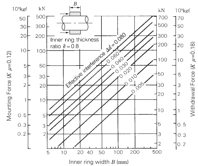
Fig. 8.5 Press-Fit and Withdrawal Forces for Inner Rings
