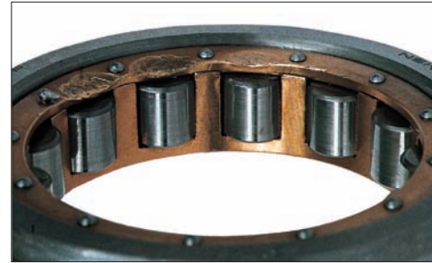
Photo 7-6 Part: Cage of a cylindrical roller bearing Symptom: Deformation of the side face of a machined high-tension-brass cage Cause: Large shock load during mounting
