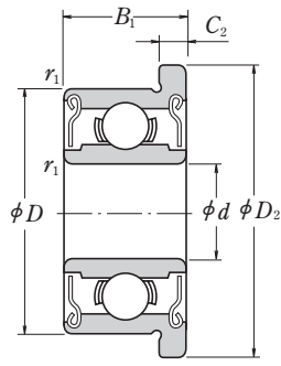
Shielded ZZ · ZZ1
