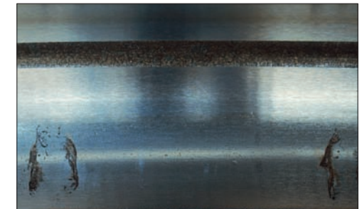
Photo 16-2 Part: Outer ring of a slewing ring Symptom: Rust on raceway surface at ball pitch Cause: Condensation during stationary periods
