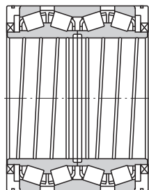
Fig. 1 Basic Design of Two-Seal Type (KVE)
