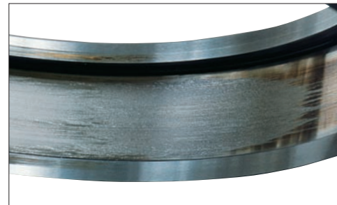
Photo 4-2 Part: Outer ring of Photo 4-1 Symptom: Smearing circumferentially on raceway surface Cause: Roller slippage due to excessive grease filling
