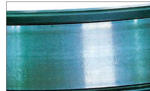
Photo 8-3 Part: Inner ring of a tapered roller bearing Symptom: Small and large indentations over entire raceway surface Cause: Debris caught in the surface
