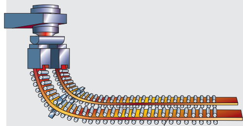
Continuous casting machine
