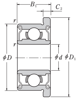
Shielded ZZ · ZS
