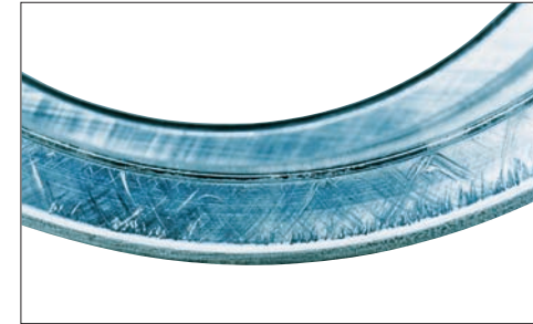
Photo 3-5 Part: Inner ring of a spherical thrust roller bearing Symptom: Scoring on the rib face of inner ring Cause: Debris caught in the surface and excessive axial load
