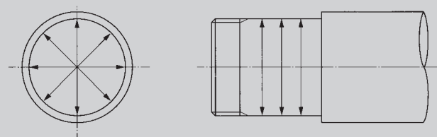
Fig. 1.21 Cylindrical Shaft
