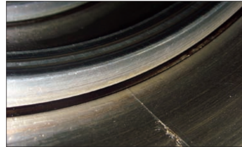
Photo 6-5 Part: Outer ring of a cylindrical roller bearing for Sendzimir mills Symptom: Fatigue crack on outer ring raceway surface Cause: Bending stress (large rotating outer ring load)
