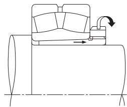
Fig. 1.16 Removal of Withdrawal Sleeve Using a Withdrawal Nut (1)
