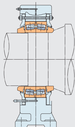
Conventional structure
