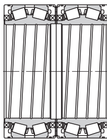
Fig. 2 Basic Design of Four-Seal Type (KVE)
