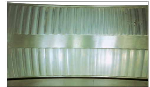
Photo 10-2 Part: Outer ring of a spherical roller bearing Symptom: Wear with a wavy or concave-and-convex texture on loaded side of raceway surface Cause: Entry of debris under repeated vibration while stationary
