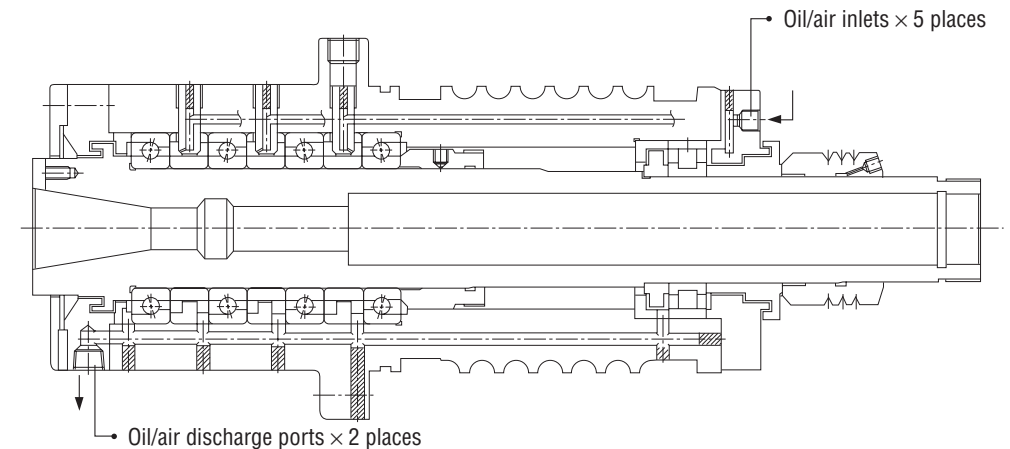
Fig. 11.10 Oil-Air Lubrication
