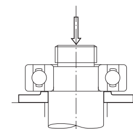
Fig. 1.12 Removal of Inner Ring Using a Press
