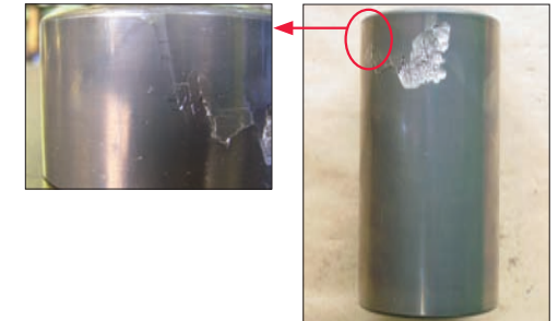
Photo 1-14 Part: Roller of a cylindrical roller bearing Symptom: Flaking of rolling surfaces Cause: Progression from a flaw or crack in roller during mounting
