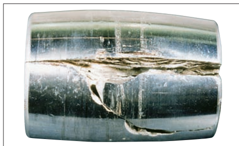
Photo 6-8 Part: Roller of a spherical roller bearing Symptom: Axial cracks on rolling surface
