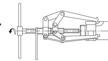
Fig. 1.14 Removal of Inner Ring Using a Withdrawal Tool (2)
