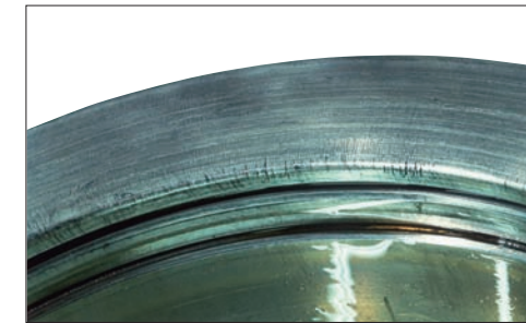
Photo 6-1 Part: Outer ring of a double-row cylindrical roller bearing Symptom: Thermal cracks on the outer ring side face Cause: Abnormal heat generation due to contact sliding between the mating part and face of outer ring
