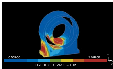
Maximum principal stress distribution
