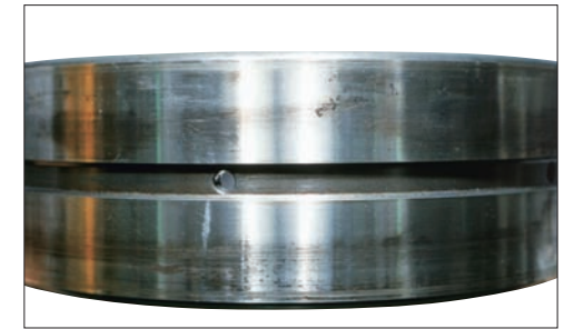
Photo 14-2 Part: Outer ring of a spherical roller bearing Symptom: Creep over entire circumference of outside surface Cause: Loose fit between outer ring and housing
