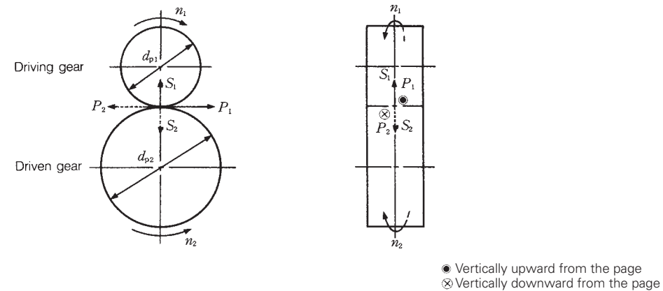
Fig. 4.47 Spur Gear
