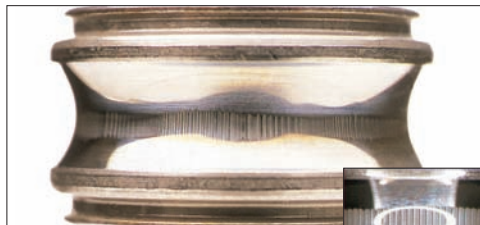
Photo 15-5 Part: Inner ring of a deep groove ball bearing Symptom: Fluting on the raceway surface (high frequency)
