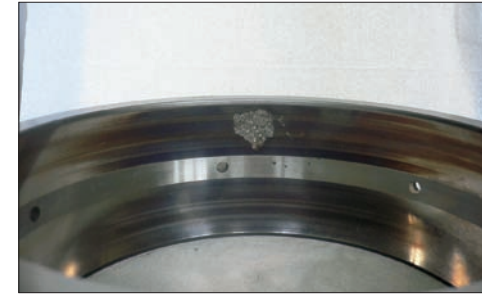
Photo 1-11 Part: Outer ring of a spherical roller bearing Symptom: Discoloration and flaking on outer ring raceway surface Cause: Poor lubrication under high temperatures
