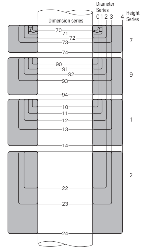
Fig. 6.7 Comparison of Cross Sections of Thrust Bearings (Excluding Diameter Series 5) for Various Dimension Series
