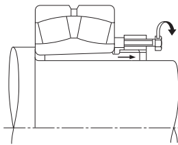
Fig. 1.17 Removal of Withdrawal Sleeve Using a Withdrawal Nut (2)
