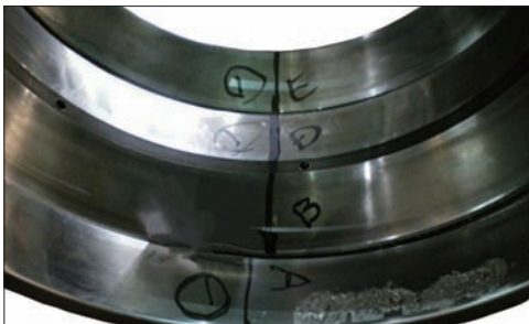
Photo 1-9 Part: Outer ring of a four-row tapered roller bearing Symptom: Flaking of raceway (loading area) Cause: Excessive moment load
